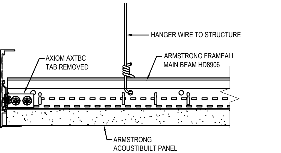
ACOUSTIC CEILING CLOUD DETAIL
