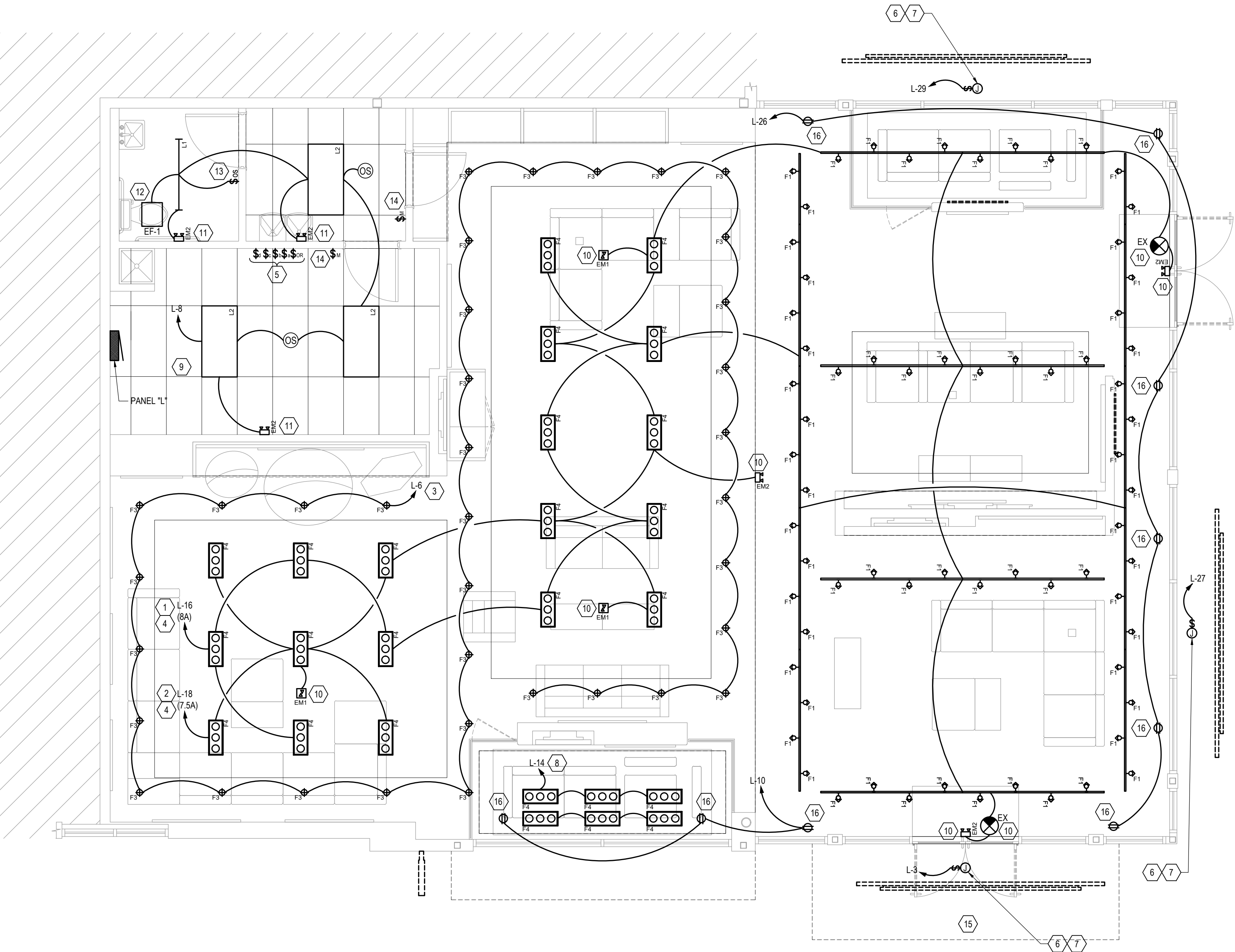
LIGHTING PLAN 1/4" = 1'-0"
