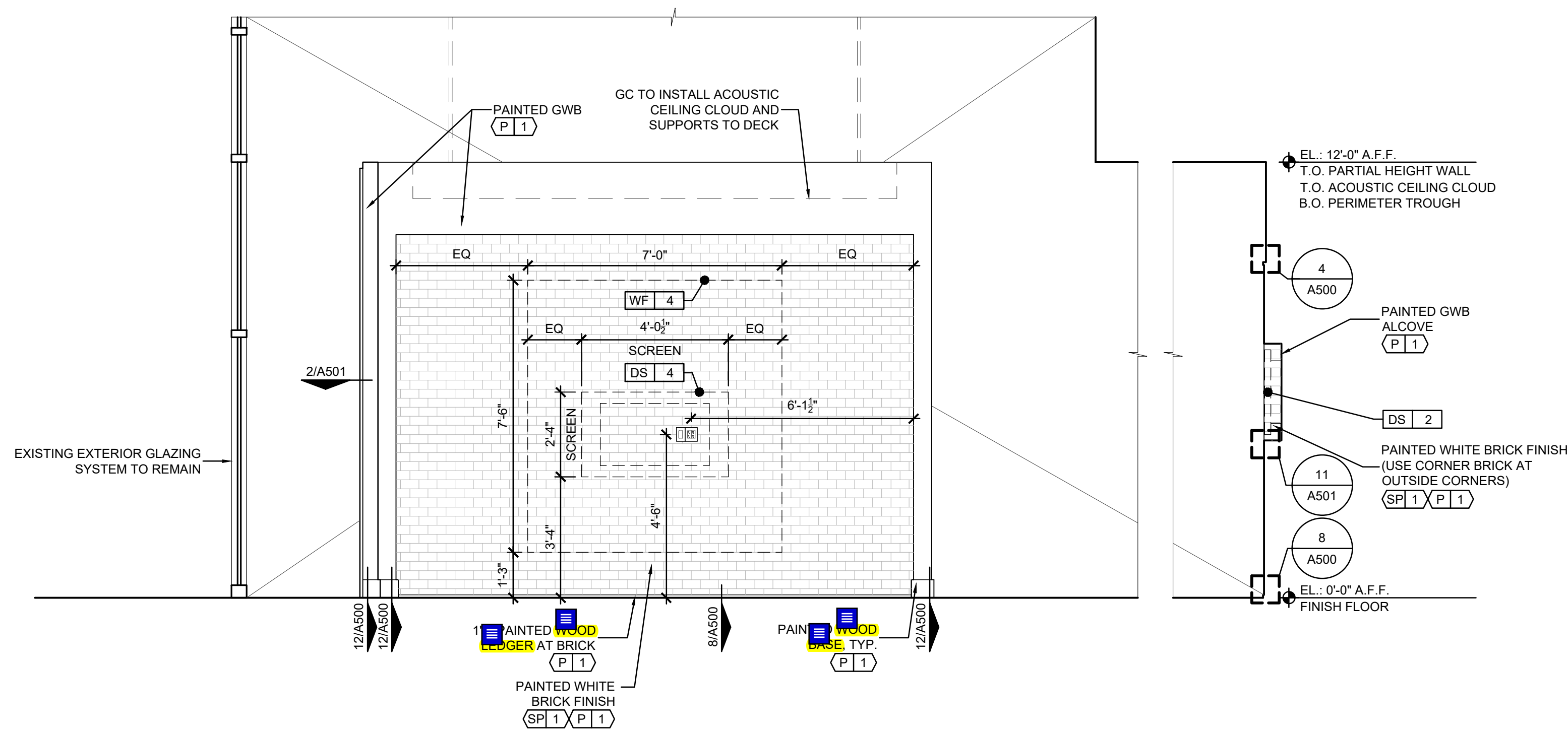
2 INTERIOR ELEVATION - SALES WF/4 WALL AND CASHWRAP
